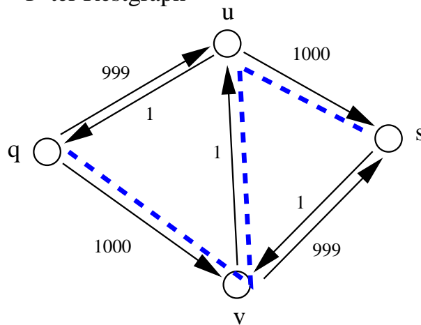
1-ter Restgraph
