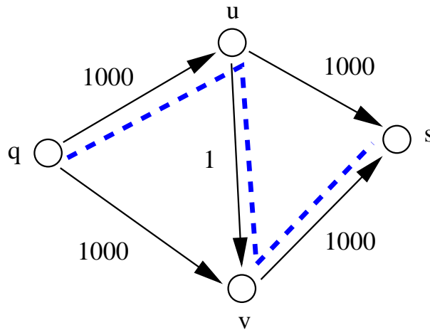
0-ter Restgraph
